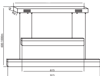
ML 401 18W LED [93W] 1260 lm
