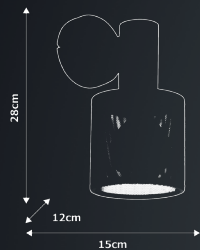
MLP 3719 1xE27 60W
