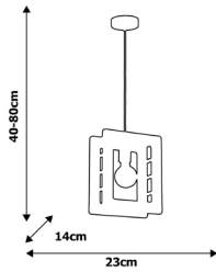
MLP 3753 1xE27 60W
