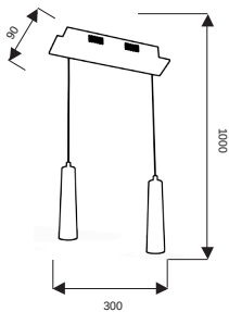
MLP 565 10W [50W] 700 lm
