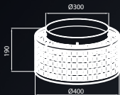
ML 369 18W LED [93W] 1260 lm
