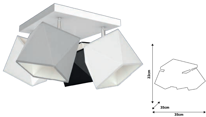
MLP 4711 1xE27 60W
