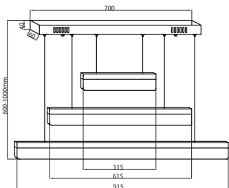
ML 403 36W LED [180W] 2520 lm
