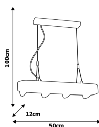
ML 3837 40W LED [200W] 2800 lm
