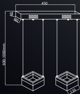
ML 445 24W [122W] 1680 lm
