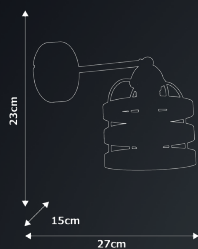
MLP 790 1xE27 60W
