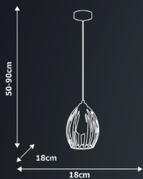
MLP 4731 1xE27 60W
