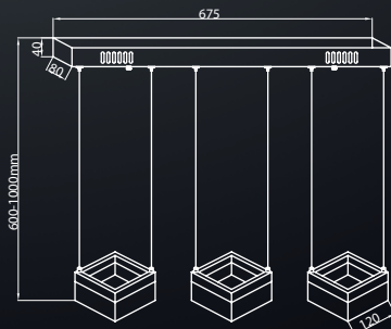
ML 446 36W LED [180W] 2520 lm
